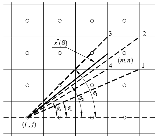
Fig. 5. Geometrical interpretation of s^*(\theta) and of angles \theta_1, \theta_2, \theta_3 and \theta_4 .
